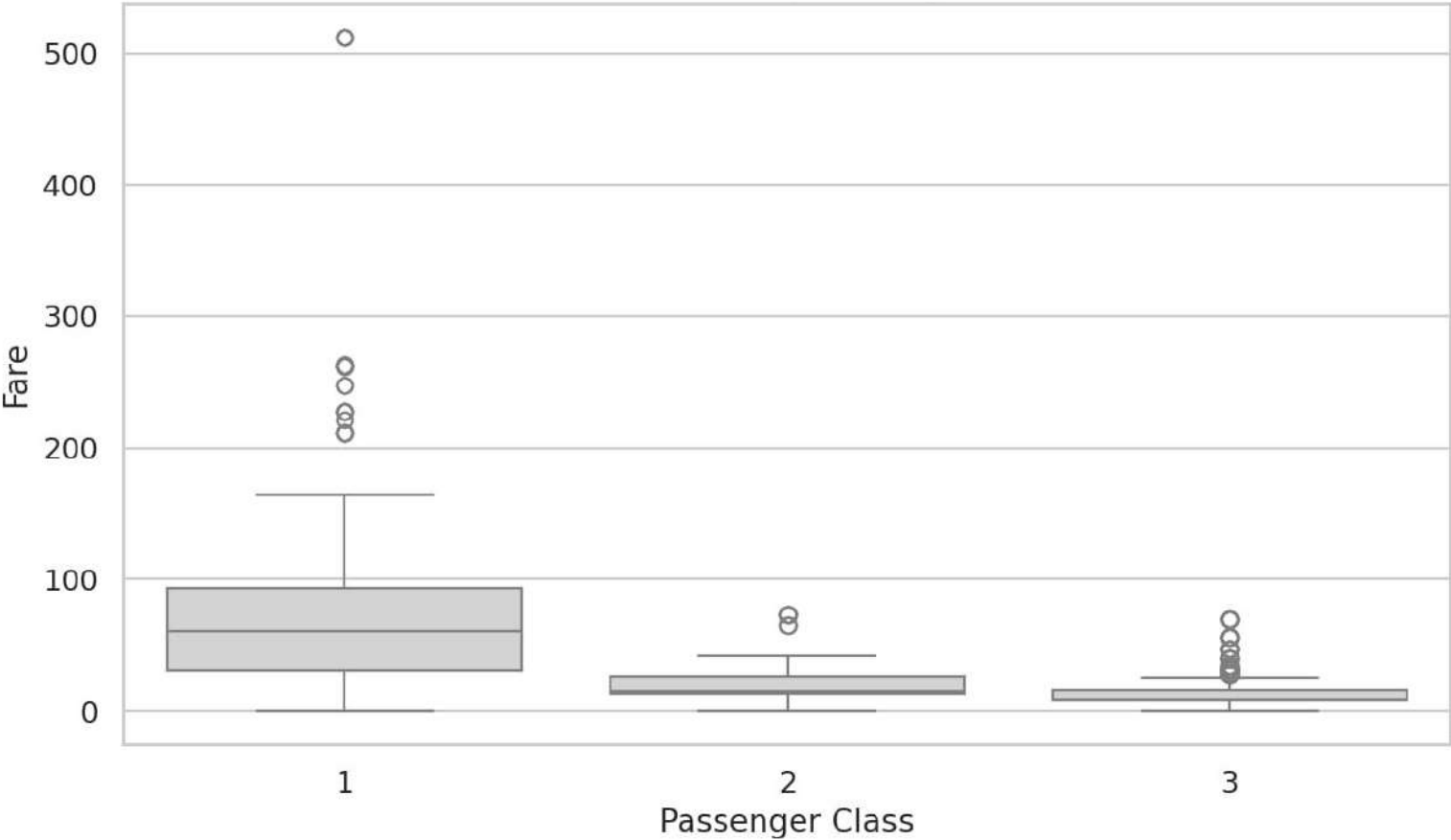
Fare Distribution by Passenger Class
