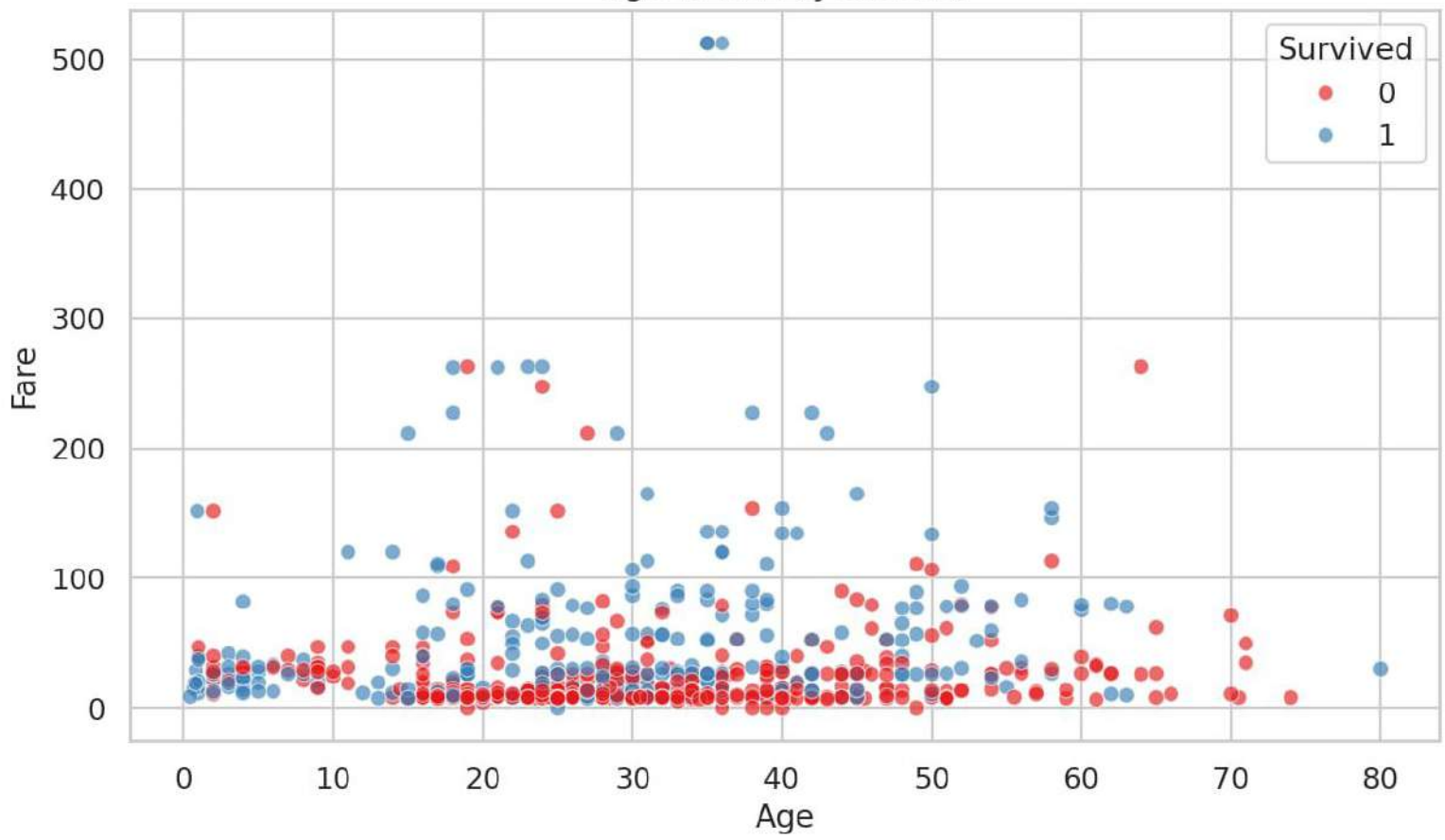
Age vs Fare by Survival
