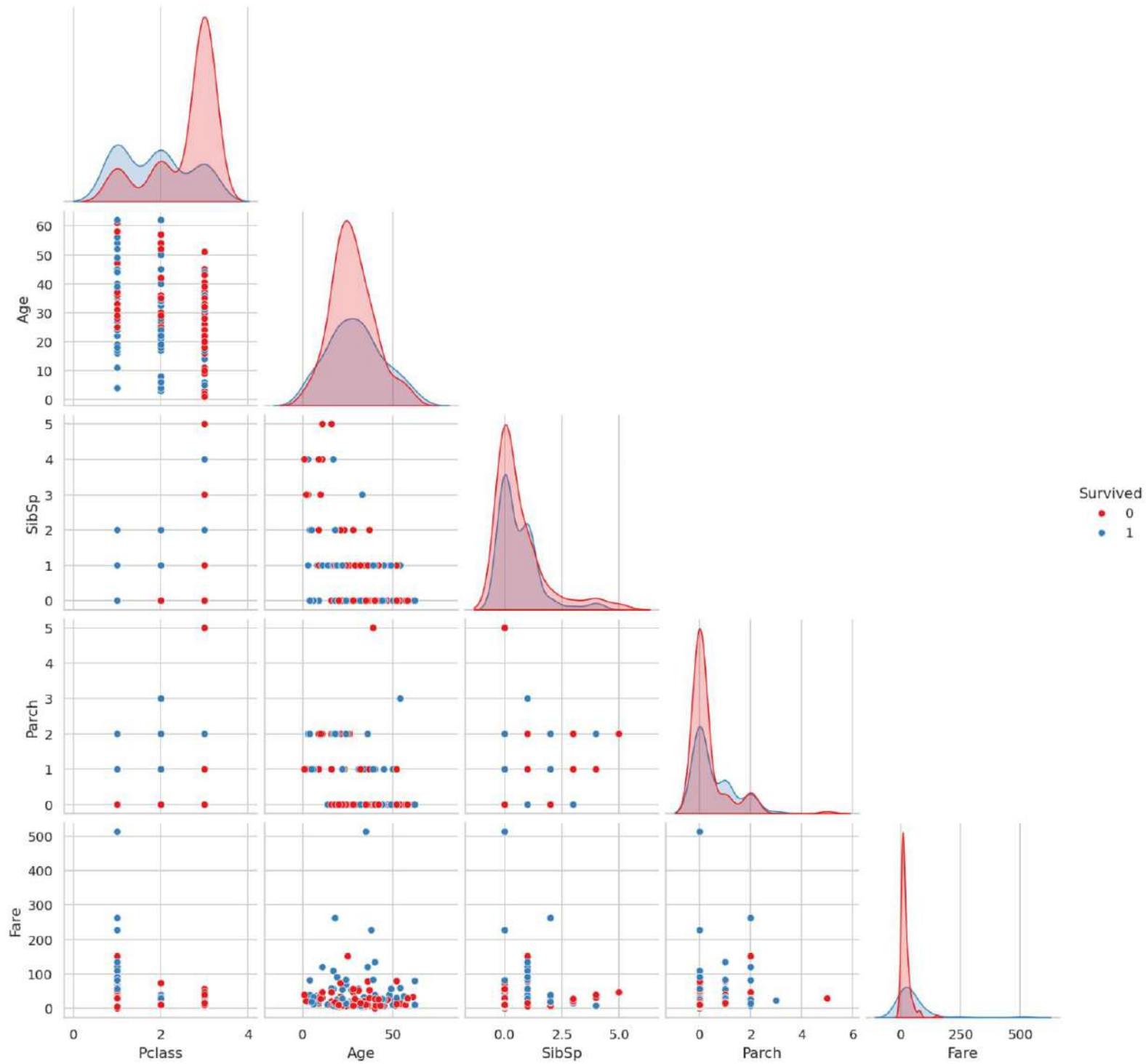
Pairplot of Key Numeric Variables
