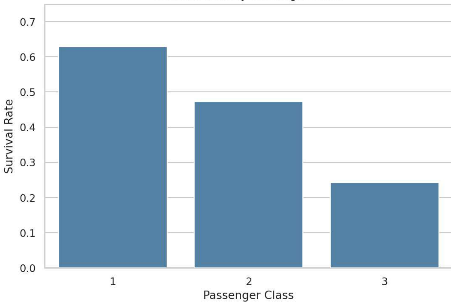
Survival Rate by Passenger Class
